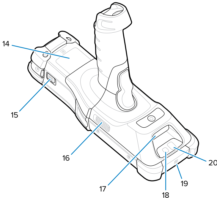
Figure 2 Bottom View
