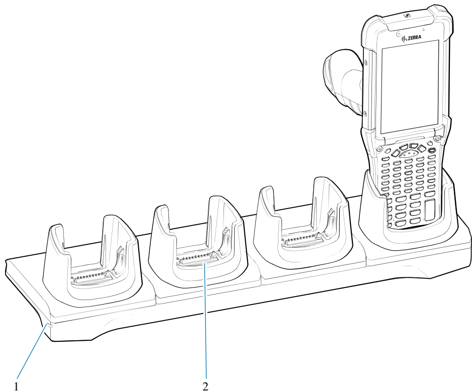
Figure 5 4-Slot Charge Only ShareCradle
